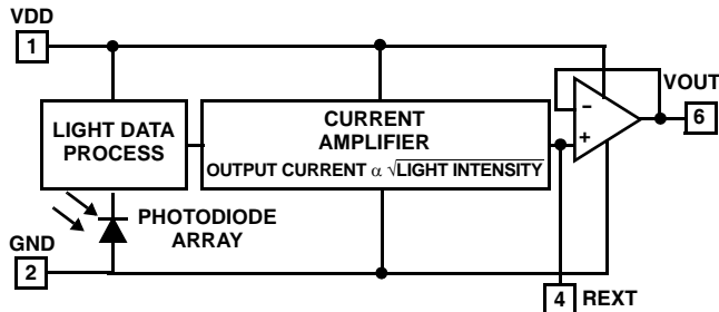
FIGURE 1. BLOCK DIAGRAM OF ISL29102 AMBIENT LIGHT SENSOR WITH INTEGRATED AMPLIFIER
