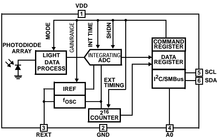
FIGURE 2. BLOCK DIAGRAM OF ISL29020, AMBIENT LIGHT SENSOR WITH ADC, AND I 2 C INTERFACE
